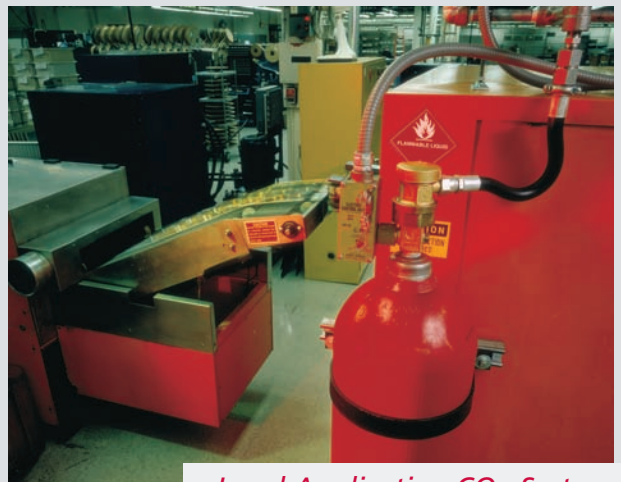
Local Application CO 2 System
